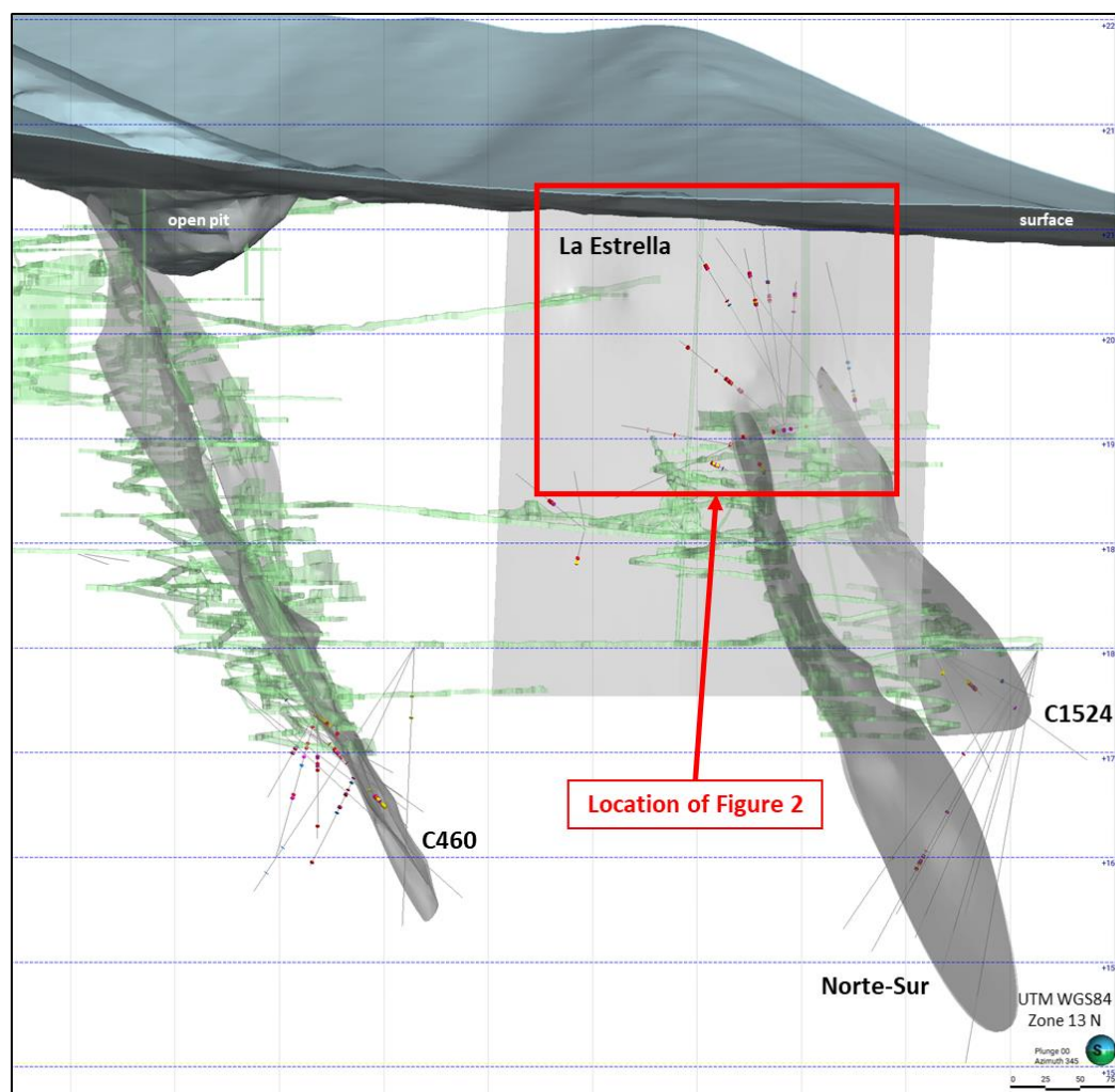
Figure 1: Cross Section View of Quebradillas Mine Toward NNW
