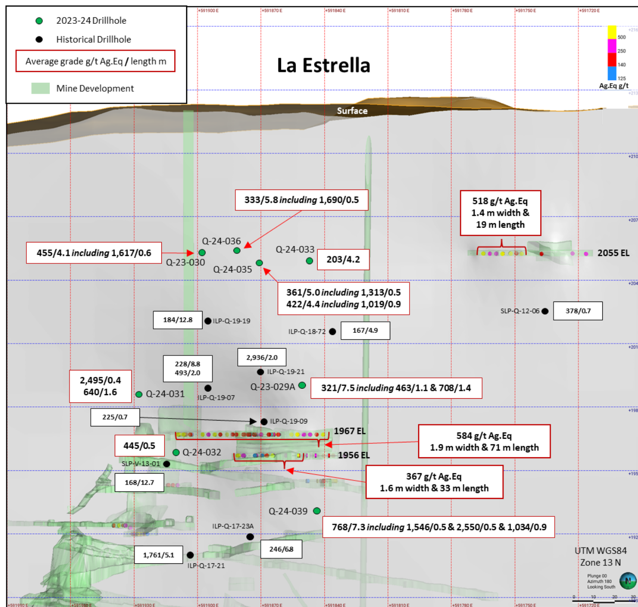
Figure 2: Longitudinal Section of La Estrella Zone View Toward South
