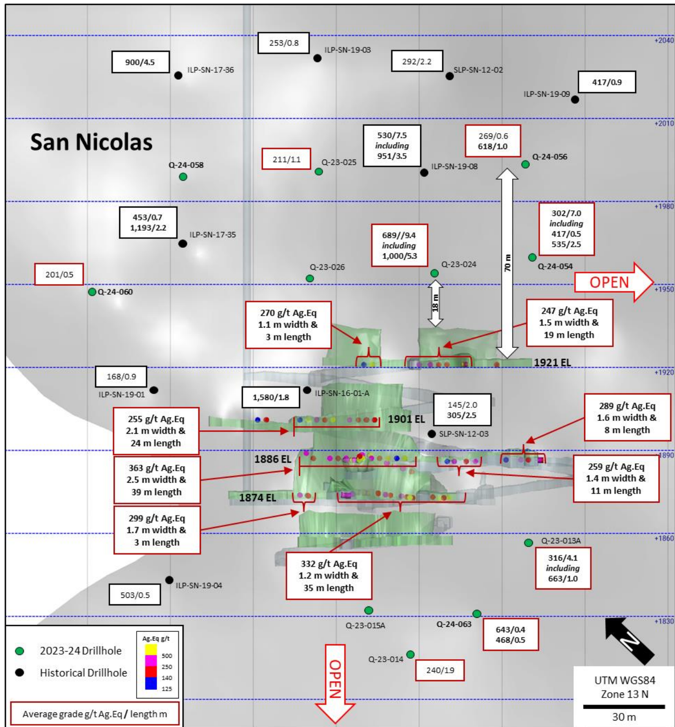
Figure 2: Longitudinal Section San Nicolas Zone View to NE.
