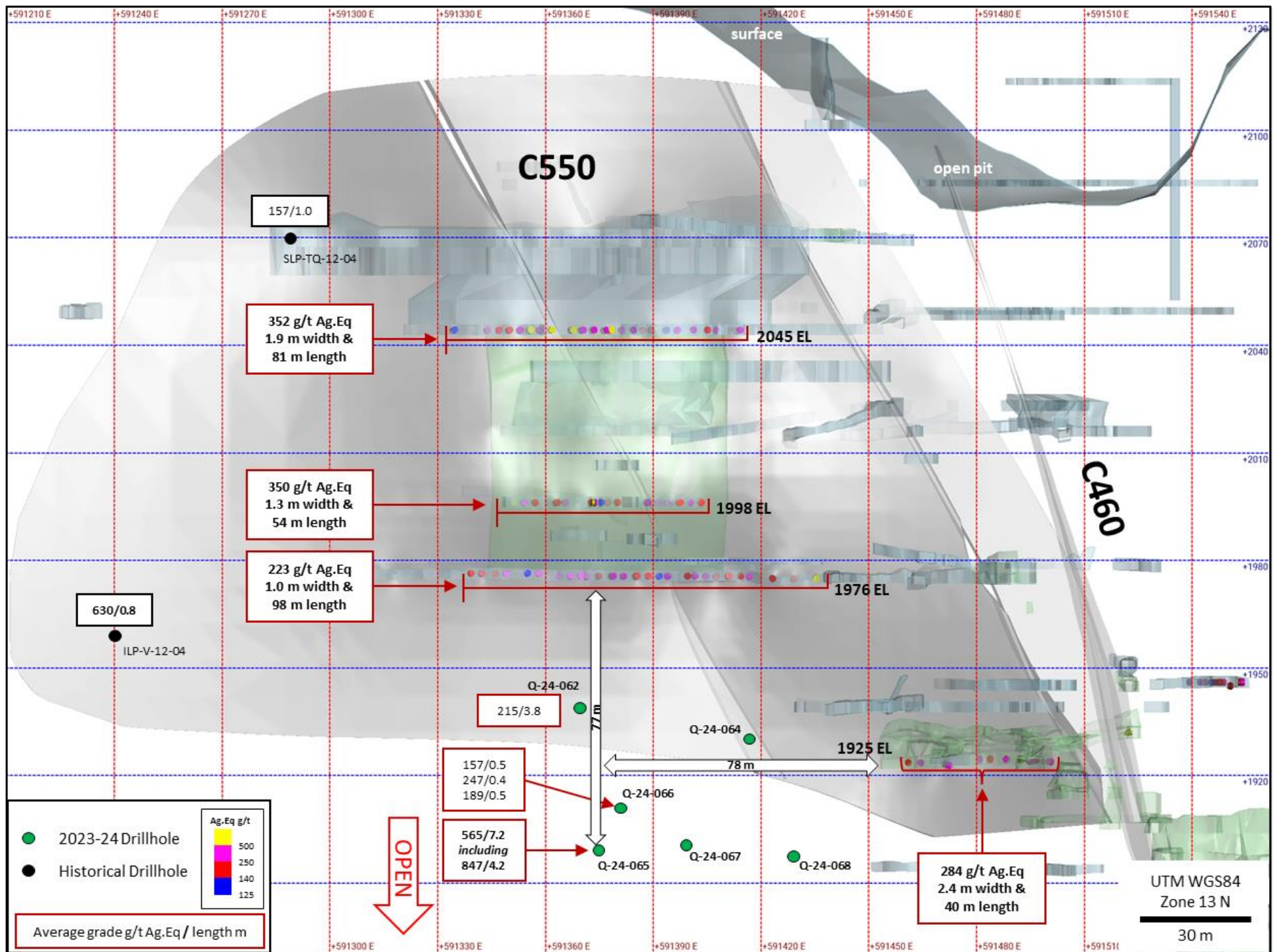
Figure 3: Longitudinal Section of C550 View to N.
